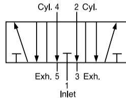
4-WAY 3-POSITION OPEN CENTER
