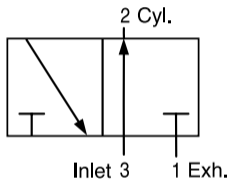
3-WAY 2-POSITION NORMALLY PASSING
