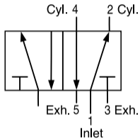
4-WAY 2-POSITION (5 PORTED)
