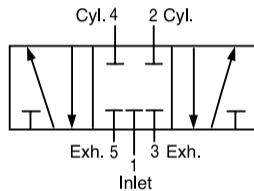
4-WAY 3-POSITION CLOSED CENTER
