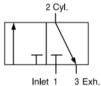
3-WAY 2-POSITION NORMALLY NON-PASSING
